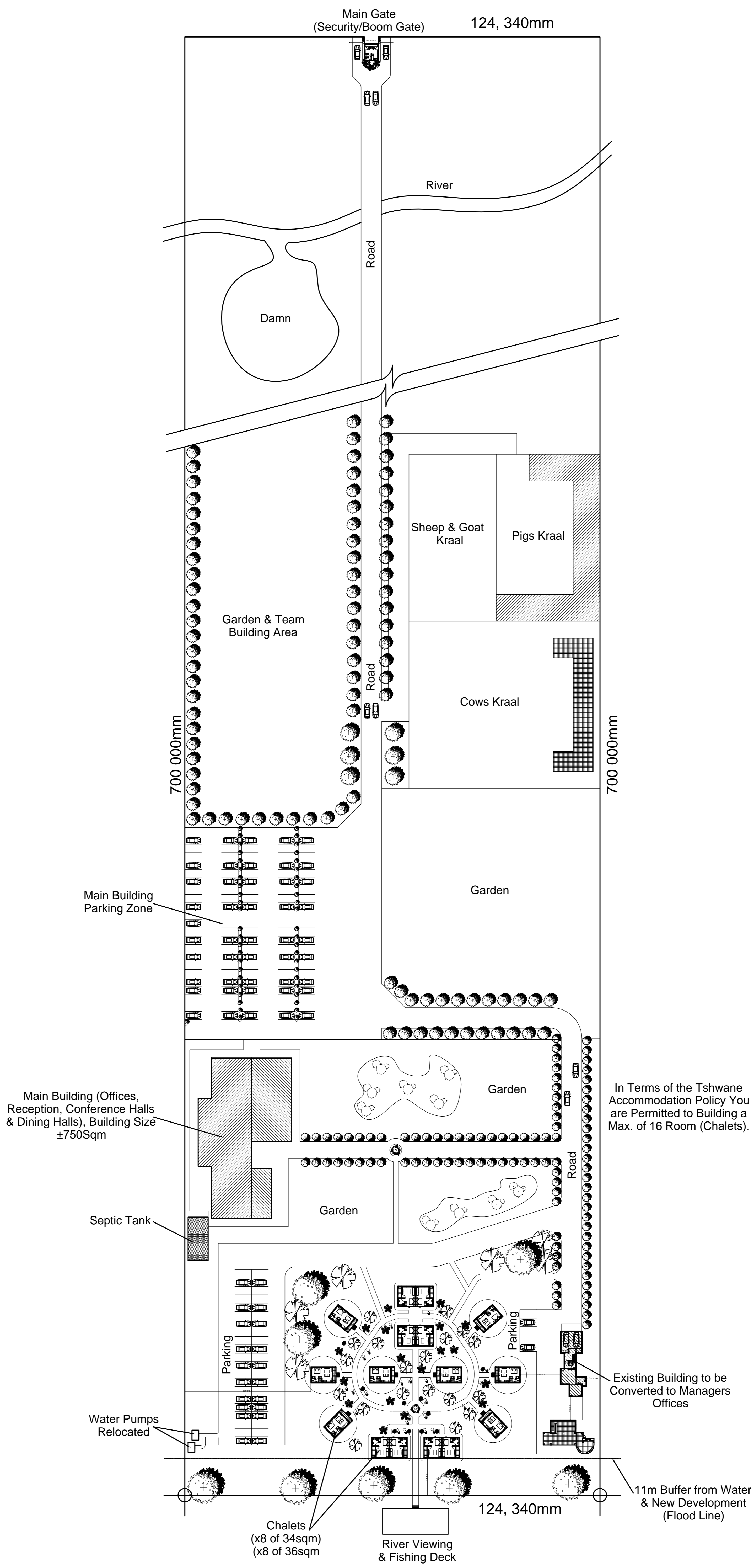
Proposed Site Layout For Development SCALE : NTS
